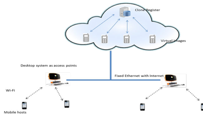
Figure 3.1. Simulation architecture
